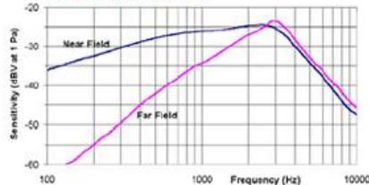
Frequency Response
