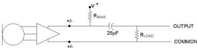
Load Circuit
