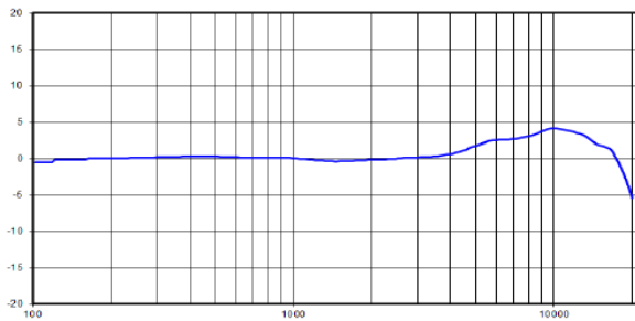
Frequency response measured at 1/4"
